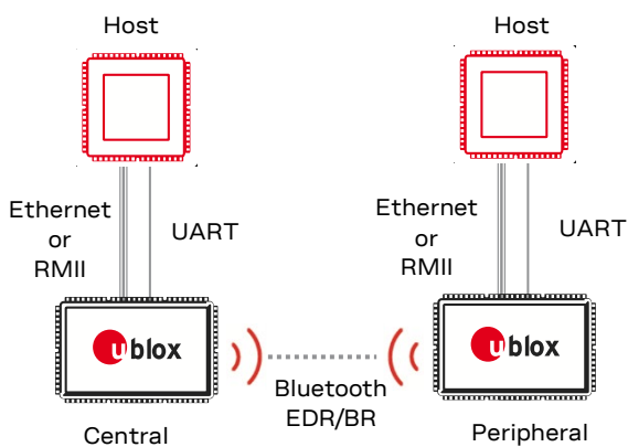
Figure 1: Bluetooth SPP connection
